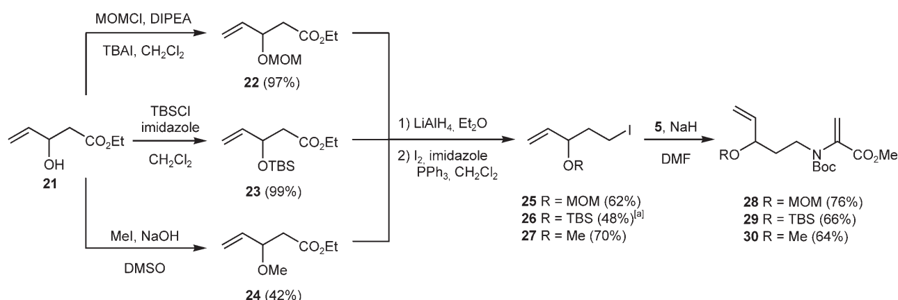
Scheme 6. Synthesis of O -substituted RCM precursors; [a] DIBALH was used for the reduction instead of LiAlH 4 .
