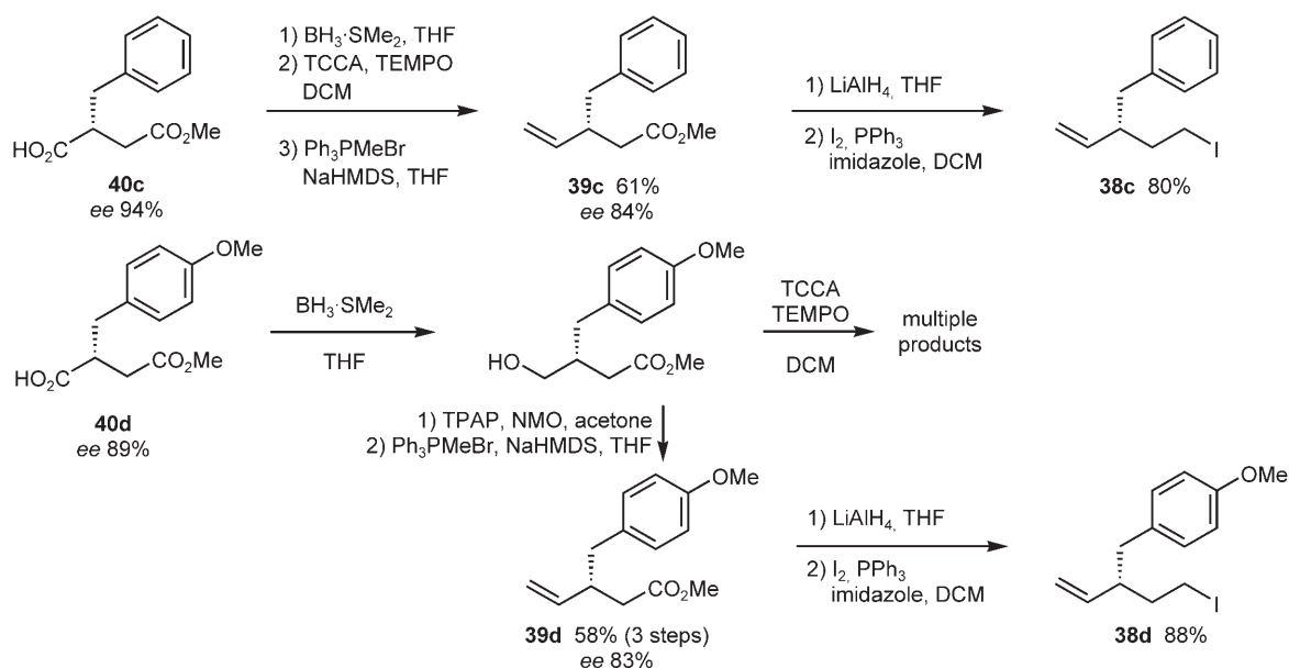
Scheme 10. Synthesis of aryl-substituted iodides.
