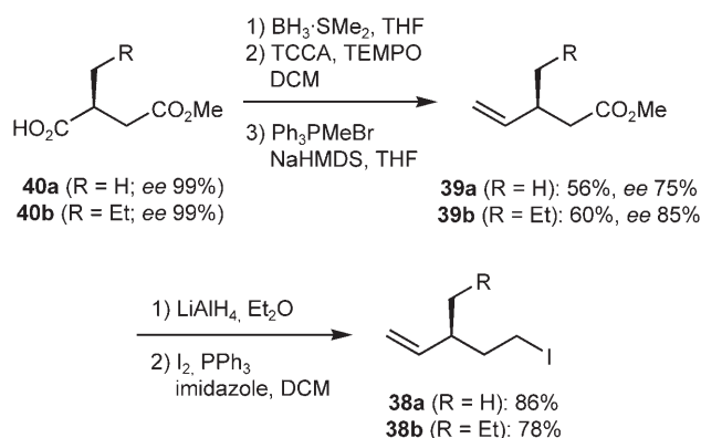
Scheme 9. Transformation of hydrogenation products into unsaturated iodides.
