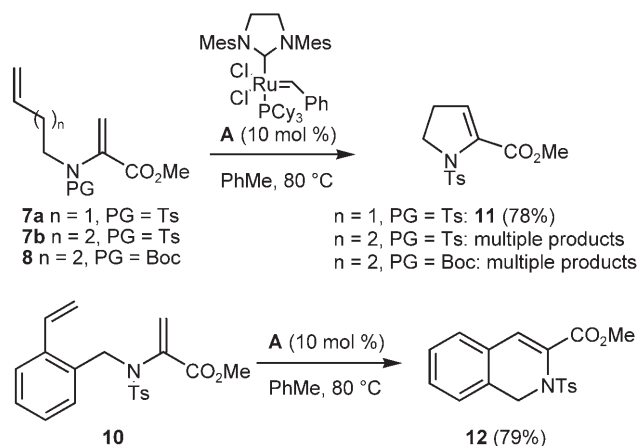
Scheme 3. RCM-mediated generation of five- and six-membered ring heterocycles.
