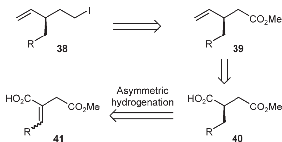
Scheme 8. Retrosynthetic approach to optically active iodide building blocks.
