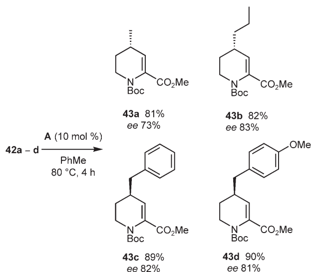
Scheme 12. Ring-closing metathesis of optically active dehydroamino acids.
