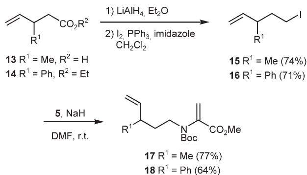
Scheme 4. Synthesis of allylically substituted RCM precursors.
