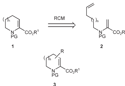
Scheme 1. Ring-closing metathesis of dehydroamino acids.
