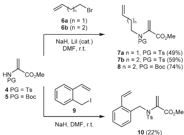
Scheme 2. Synthesis of RCM precursors via alkylation of protected dehydroalanine methyl esters.
