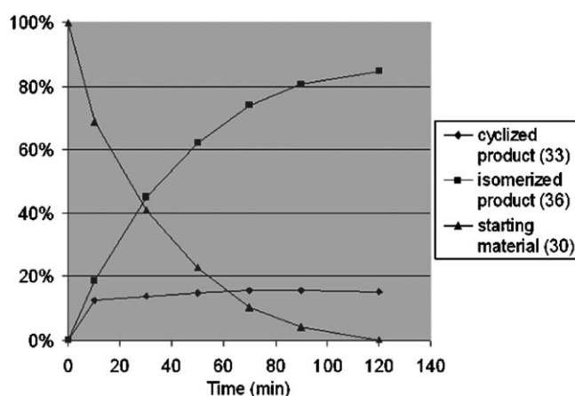
Figure 2. Conditions: 30 in C 6 D 6 (5 μM), A (10 mol %), 70°C. Values are based on 1 H NMR.
