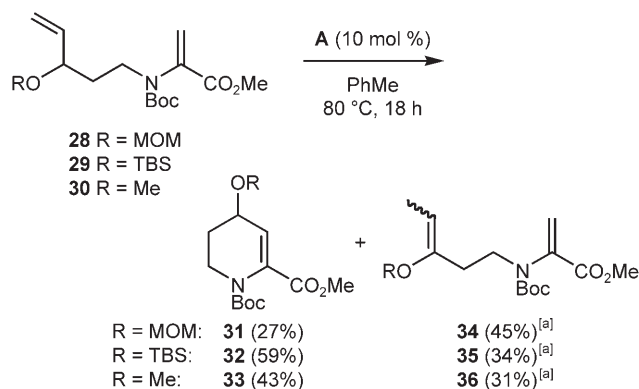
Scheme 7. RCM and isomerization of allylic ether fragments; [a] mixture of E/Z -isomers.
