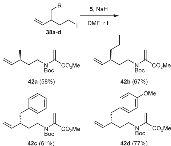
Scheme 11. Preparation of optically active RCM precursors.
