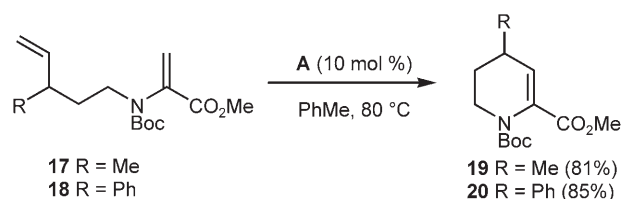
Scheme 5. RCM of allylically substituted dehydroamino acid-based precursors.
